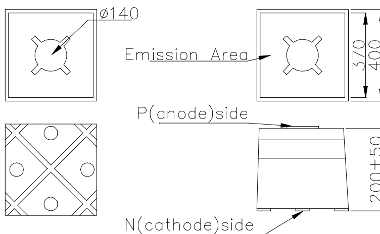
Fig.1 Electrode Pattern
