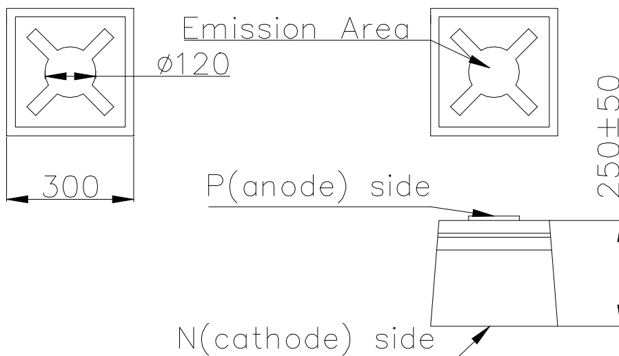
Fig.1 Electrode Pattern
