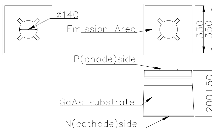
Fig.1 Electrode Pattern
