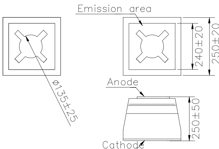
Fig.1 Electrode Pattern
