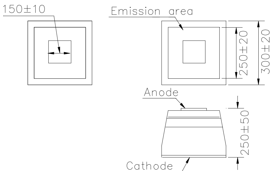
Fig.1 Electrode Pattern
