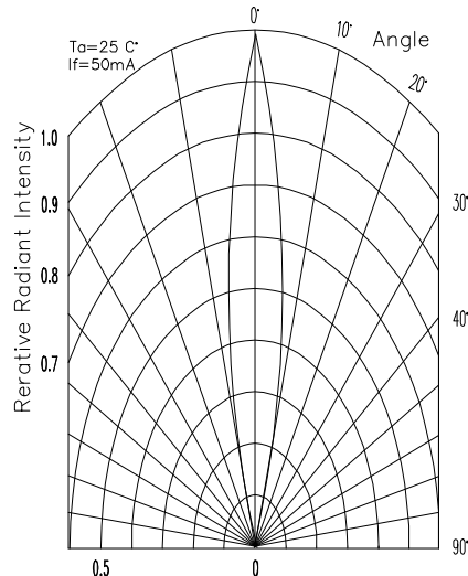
Radiation Pattern Mold type 02
