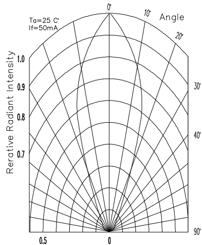
Radiation Pattern Mold type 33
