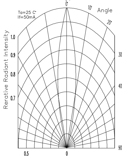
Radiation Pattern Mold type 36
