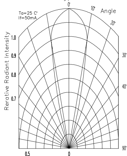
Radiation Pattern Mold type 03
