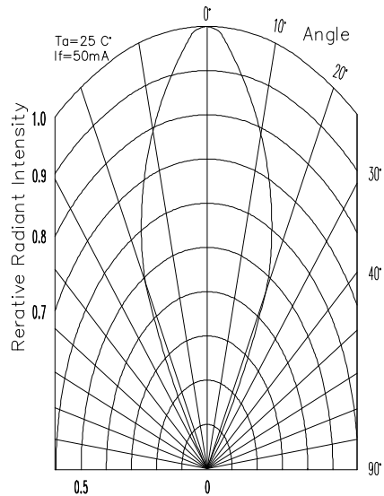
Radiation Pattern Mold type 33
