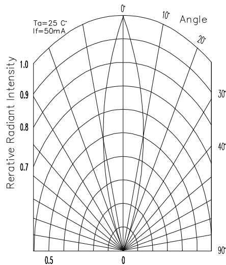
Radiation Pattern Mold type 01
