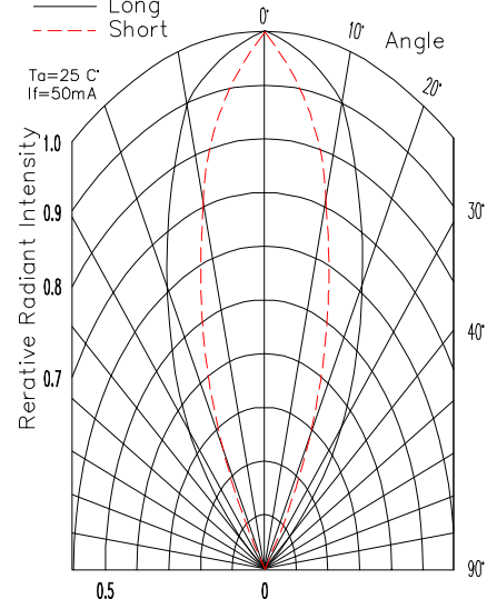
Radiation Pattern Mold type 09
